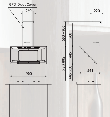
FR-SC2090V (Ventilating) [mm]
