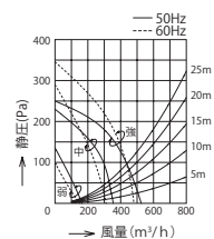
[靜壓-風量曲線]
