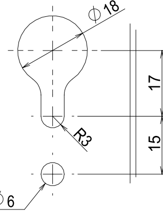
Detail: Installation hole
