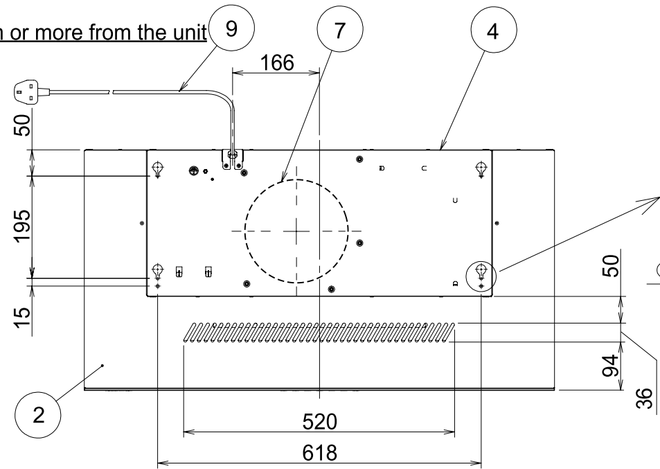
Detail: Installation hole
