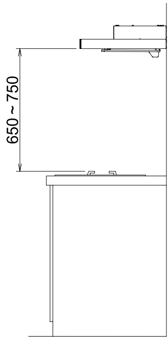
Standard Installation
