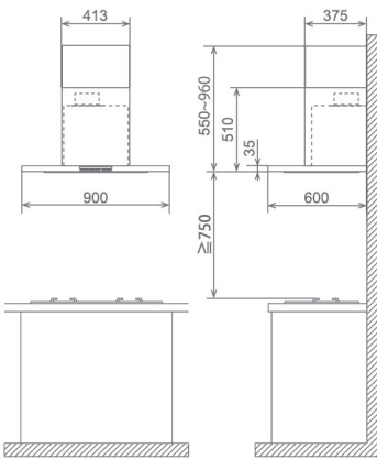
FR-CL1890V (Ventilating) [mm]
