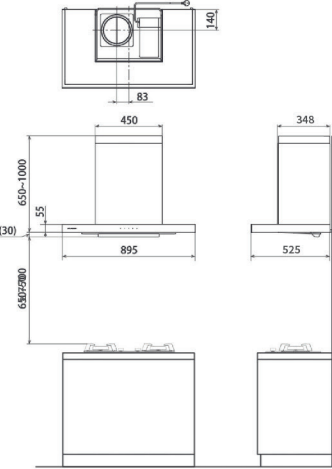
FR-ST2190V (Ventilating) [mm]
