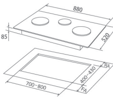
FH-GS7030 SVGL [mm]
