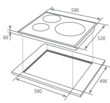
FH-ID5130 [mm]
