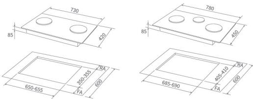
FH-GS2020 SVGL [mm]
