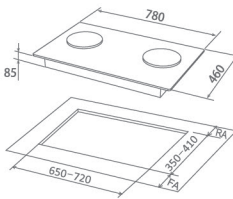
FH-GS7020 SVGL [mm]
