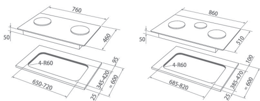
FH-GS6020 SVSS [mm]
