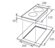
FH-ID5125 [mm]
