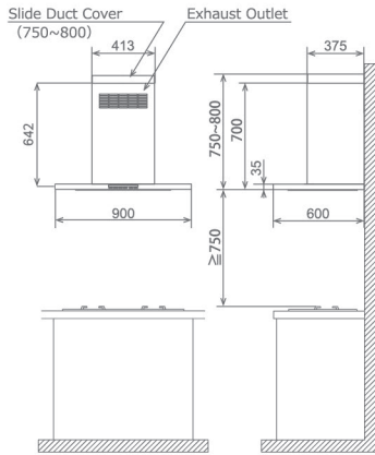
FR-CL1890R (Recycling) [mm]
