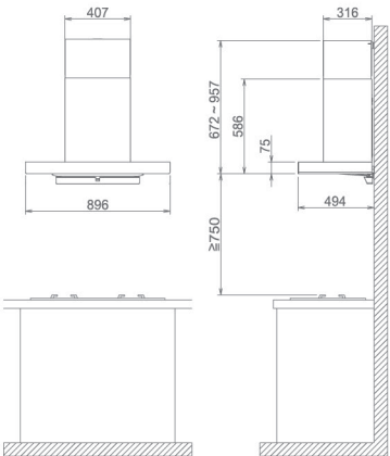
FR-LT2290V (Ventilating) [mm]
