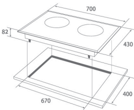
FH-IC6020 [mm]
