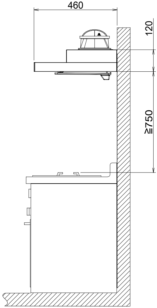
Standard Installation
