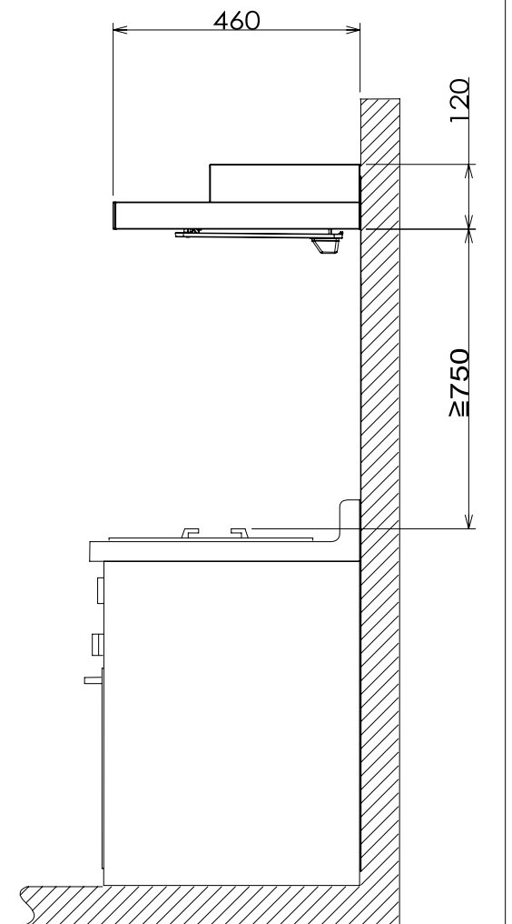
Standard Installation
