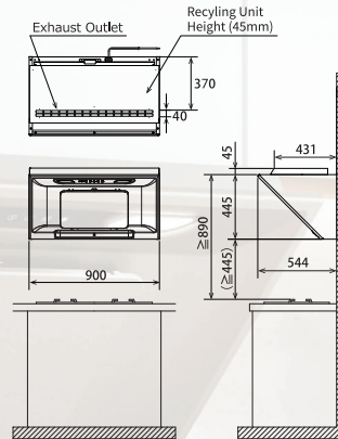
FR-SC2090R (Recycling) [mm]
