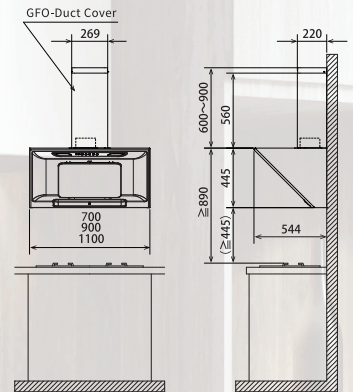
FR-SC2090V (Ventilating) [mm]
