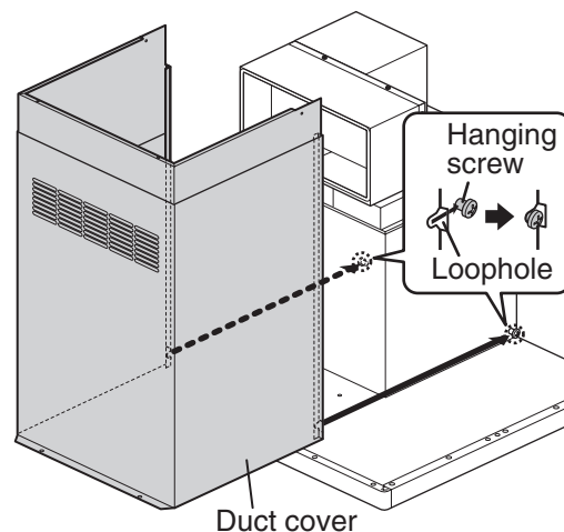
(Recycling type)
