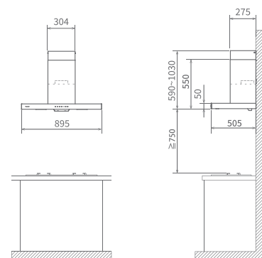
FR-HT2190V (Ventilating) [mm]
