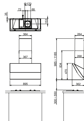
FR-SD2290V (Ventilating) [mm]
